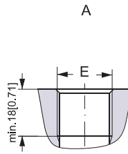
A: G Main port E: ISO 228/1 – G 1
